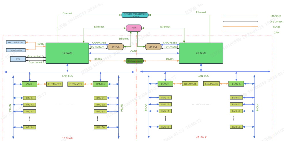
Fig5. BMS Architecture Diagram(For reference)
