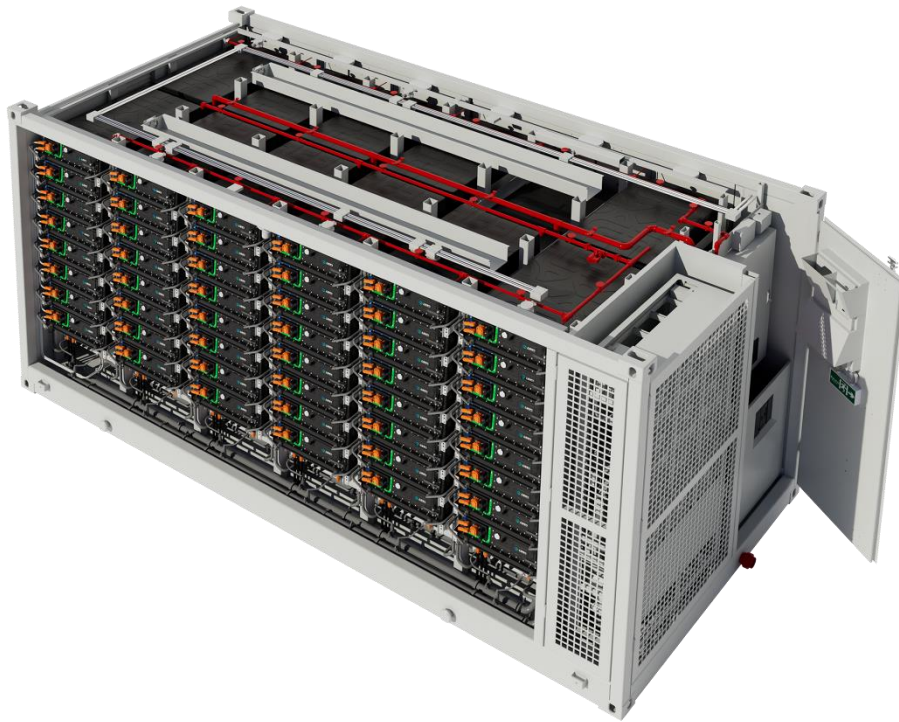
Fig4. Outside View of 5MWh Battery Container
